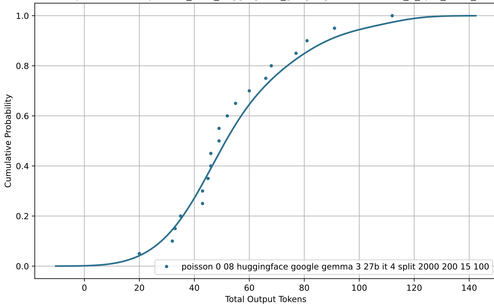
CDF of Total Output Tokens for poisson_0-08_huggingface_google-gemma-3-27b-it_4_split_2000_200_15_100
