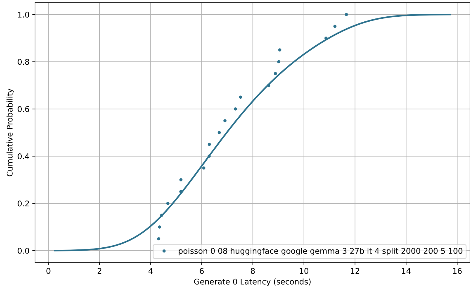
CDF of Generate 0 Latency for poisson_0-08_huggingface_google-gemma-3-27b-it_4_split_2000_200_5_100
