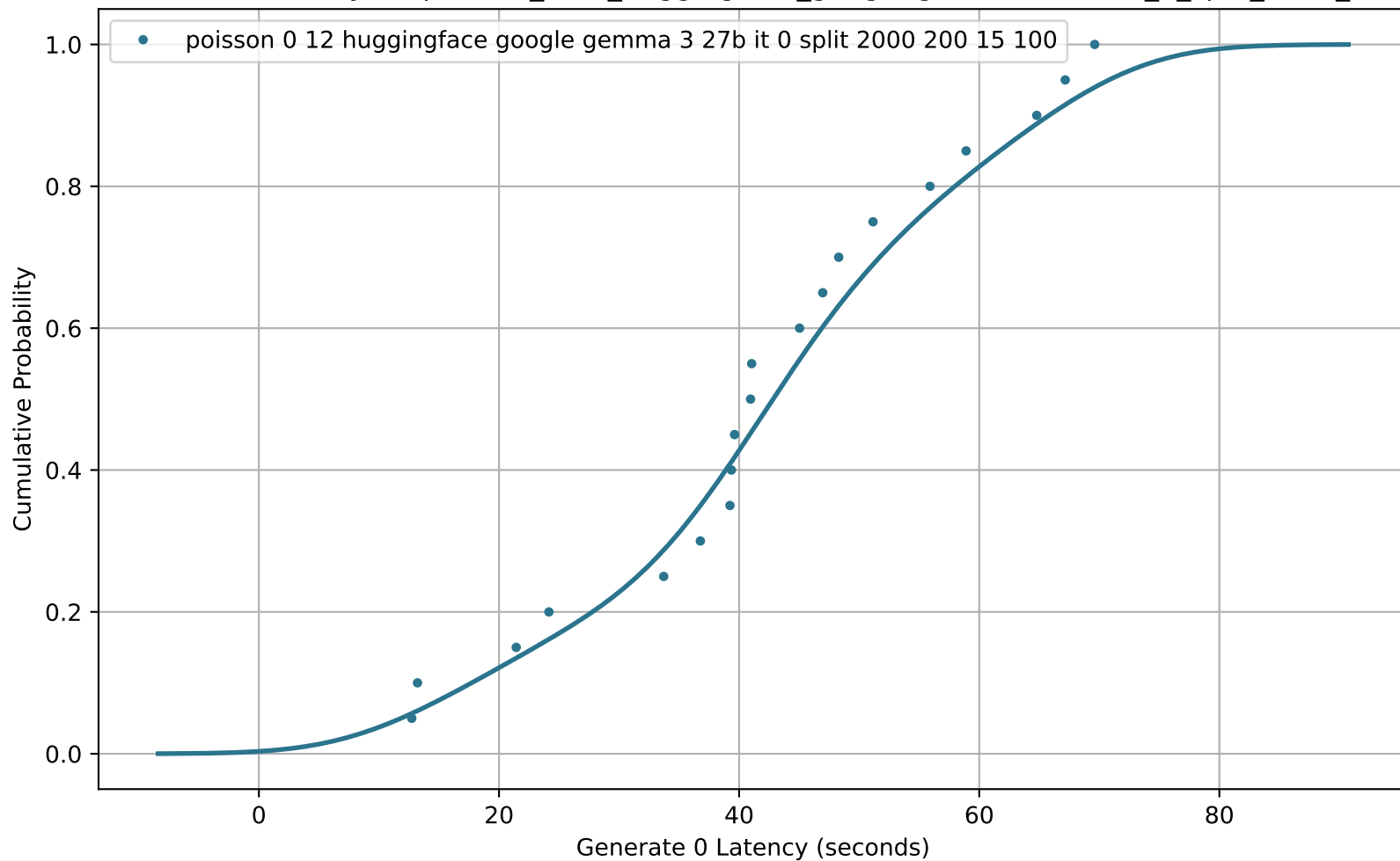
CDF of Generate 0 Latency for poisson_0-12_huggingface_google-gemma-3-27b-it_0_split_2000_200_15_100
