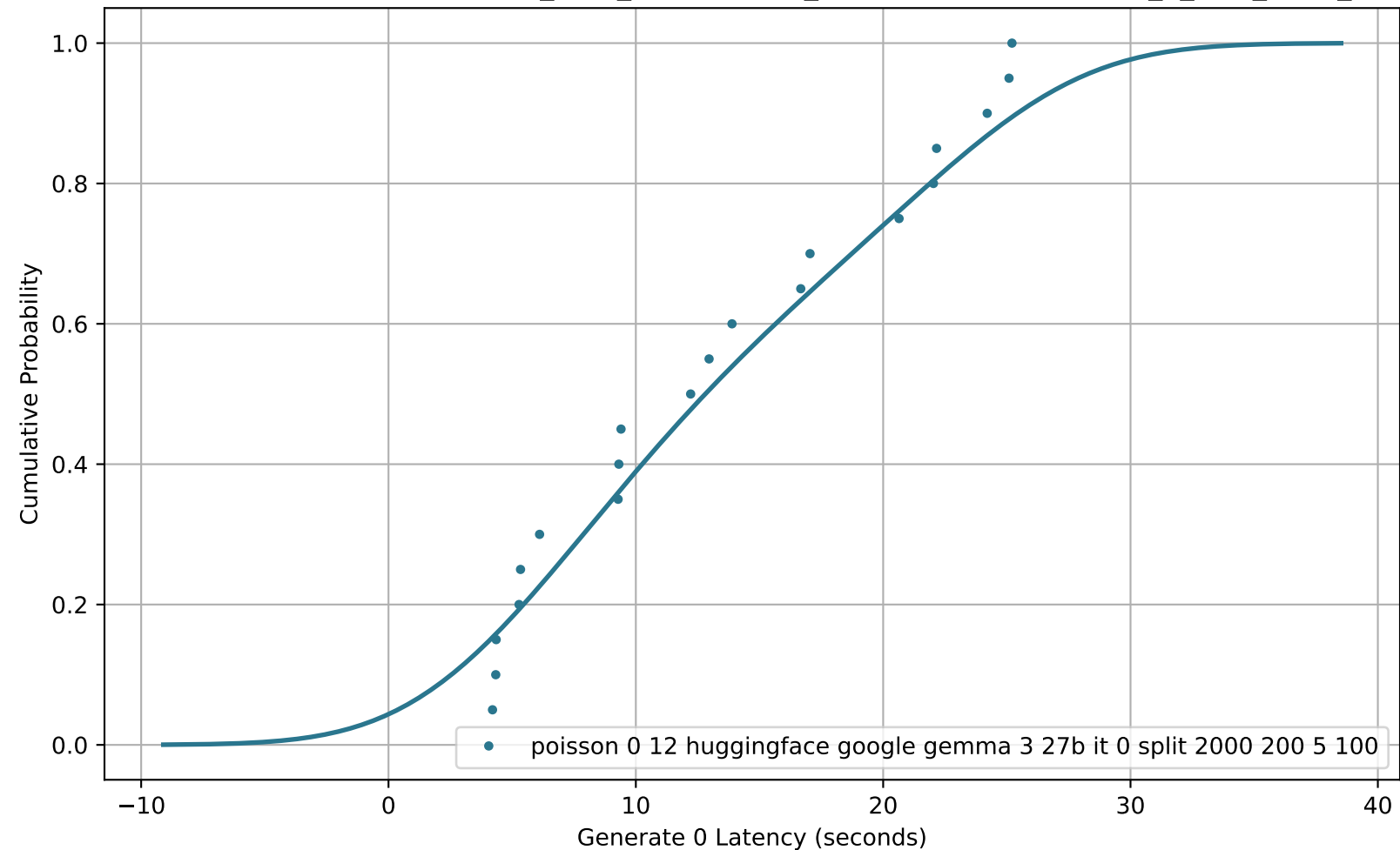
CDF of Generate 0 Latency for poisson_0-12_huggingface_google-gemma-3-27b-it_0_split_2000_200_5_100
