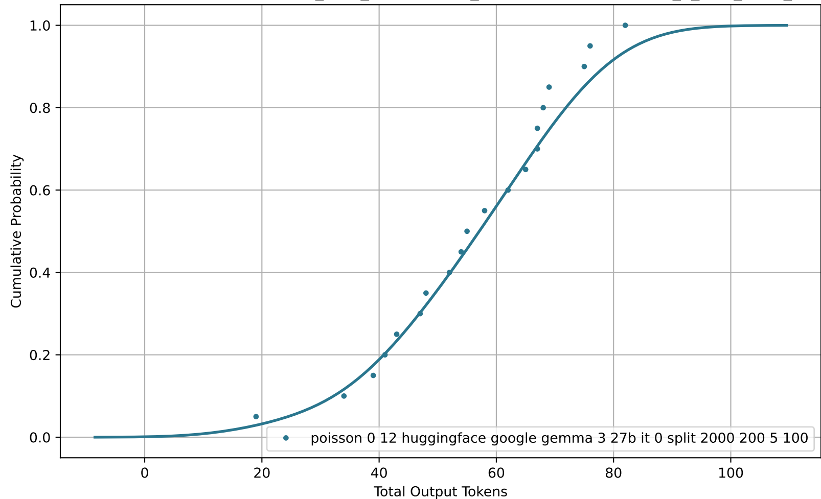
CDF of Total Output Tokens for poisson_0-12_huggingface_google-gemma-3-27b-it_0_split_2000_200_5_100
