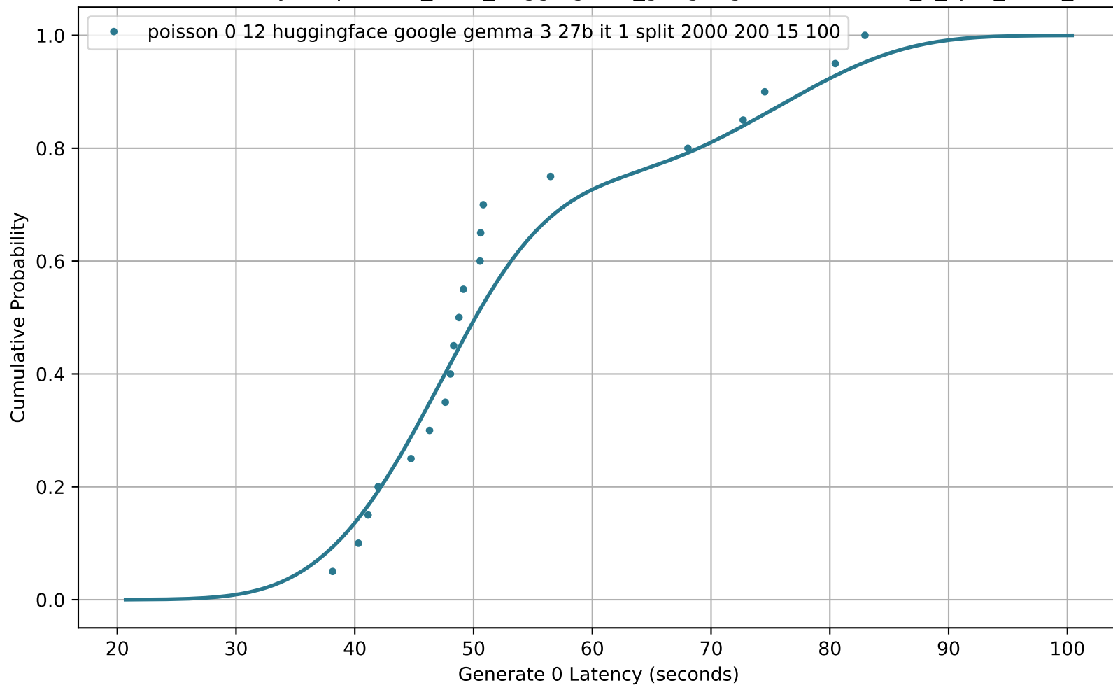
CDF of Generate 0 Latency for poisson_0-12_huggingface_google-gemma-3-27b-it_1_split_2000_200_15_100
