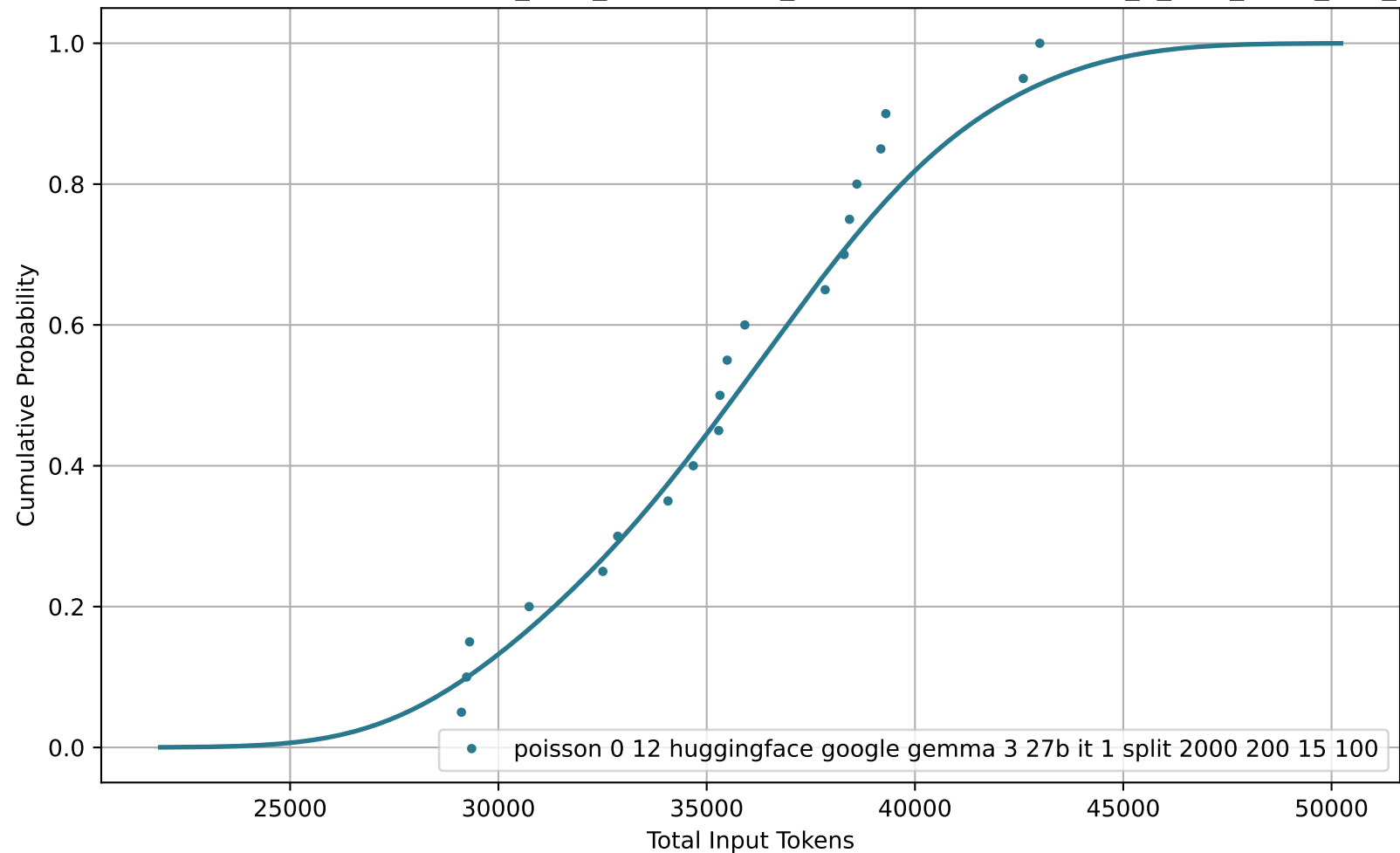
CDF of Total Input Tokens for poisson_0-12_huggingface_google-gemma-3-27b-it_1_split_2000_200_15_100
