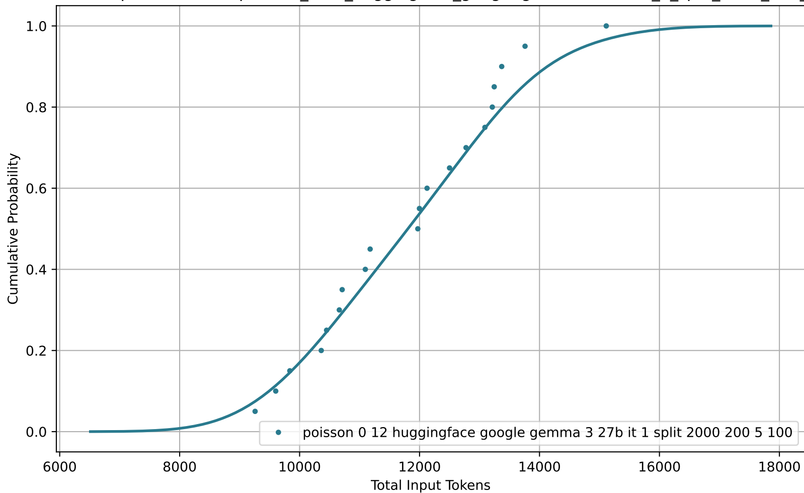
CDF of Total Input Tokens for poisson_0-12_huggingface_google-gemma-3-27b-it_1_split_2000_200_5_100
