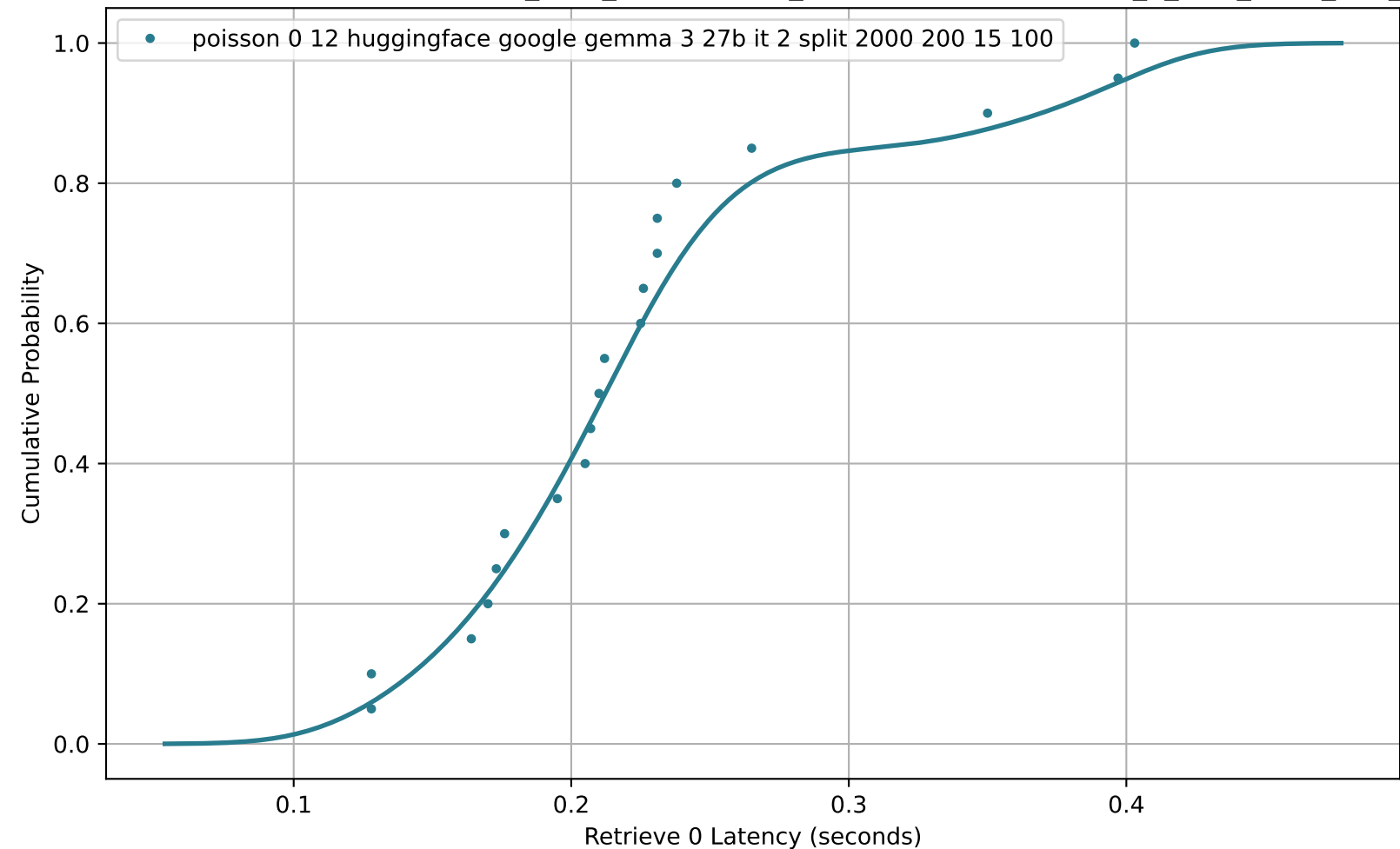
CDF of Retrieve 0 Latency for poisson_0-12_huggingface_google-gemma-3-27b-it_2_split_2000_200_15_100
