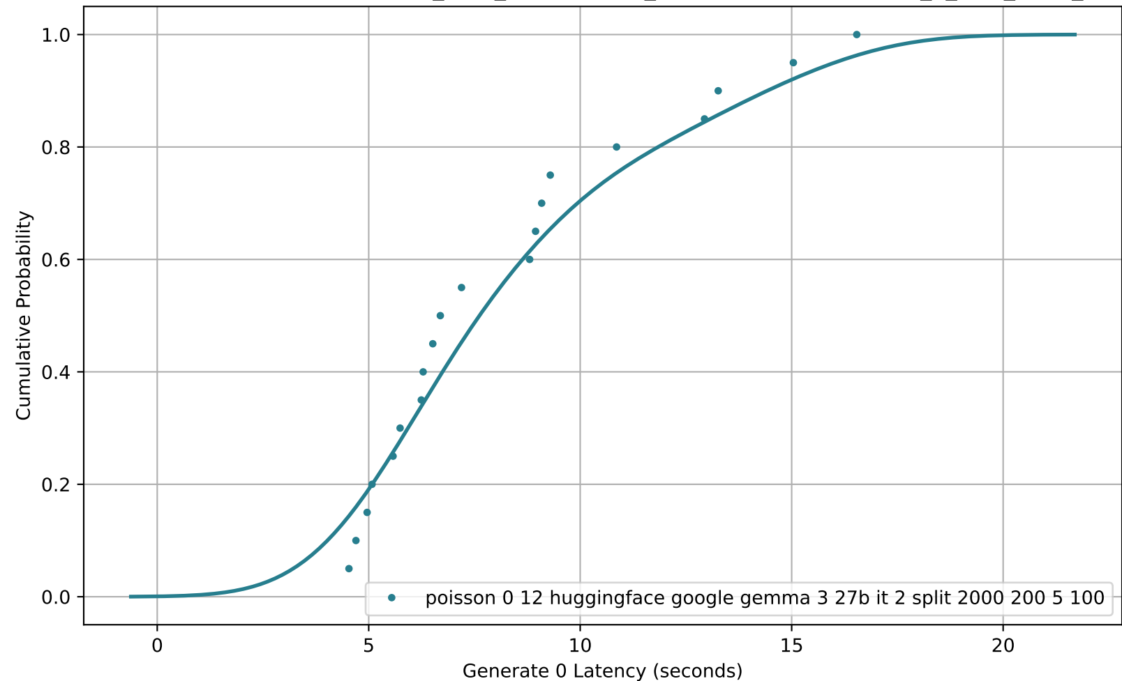
CDF of Generate 0 Latency for poisson_0-12_huggingface_google-gemma-3-27b-it_2_split_2000_200_5_100
