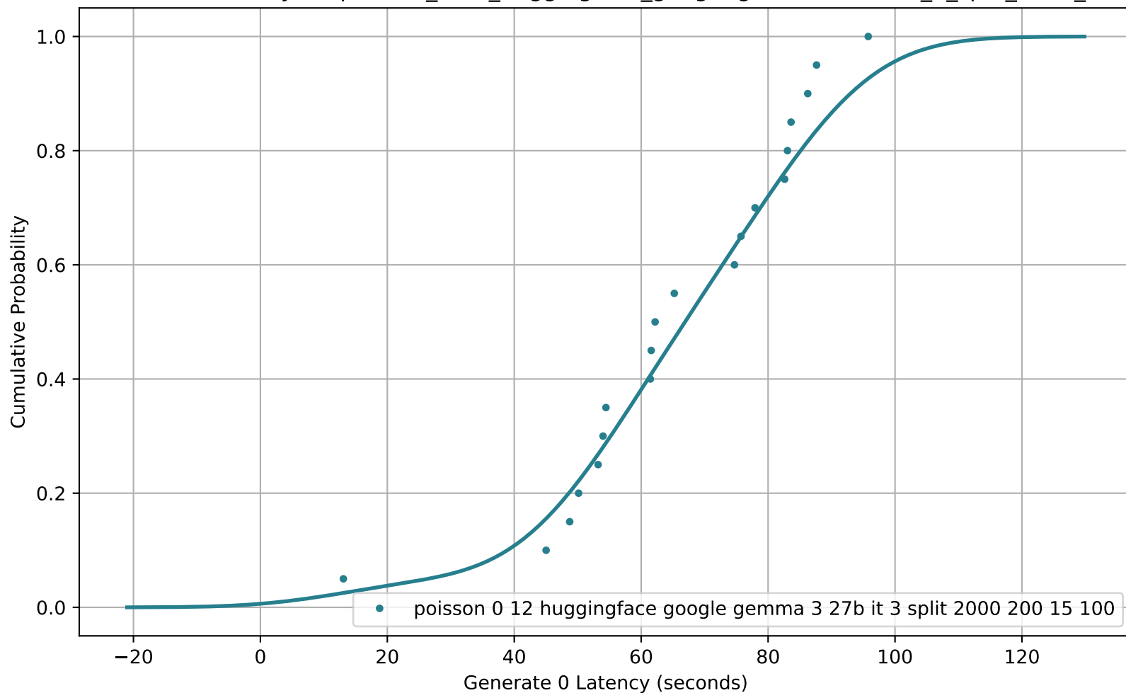
CDF of Generate 0 Latency for poisson_0-12_huggingface_google-gemma-3-27b-it_3_split_2000_200_15_100
