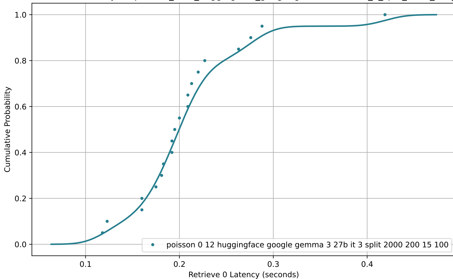
CDF of Retrieve 0 Latency for poisson_0-12_huggingface_google-gemma-3-27b-it_3_split_2000_200_15_100
