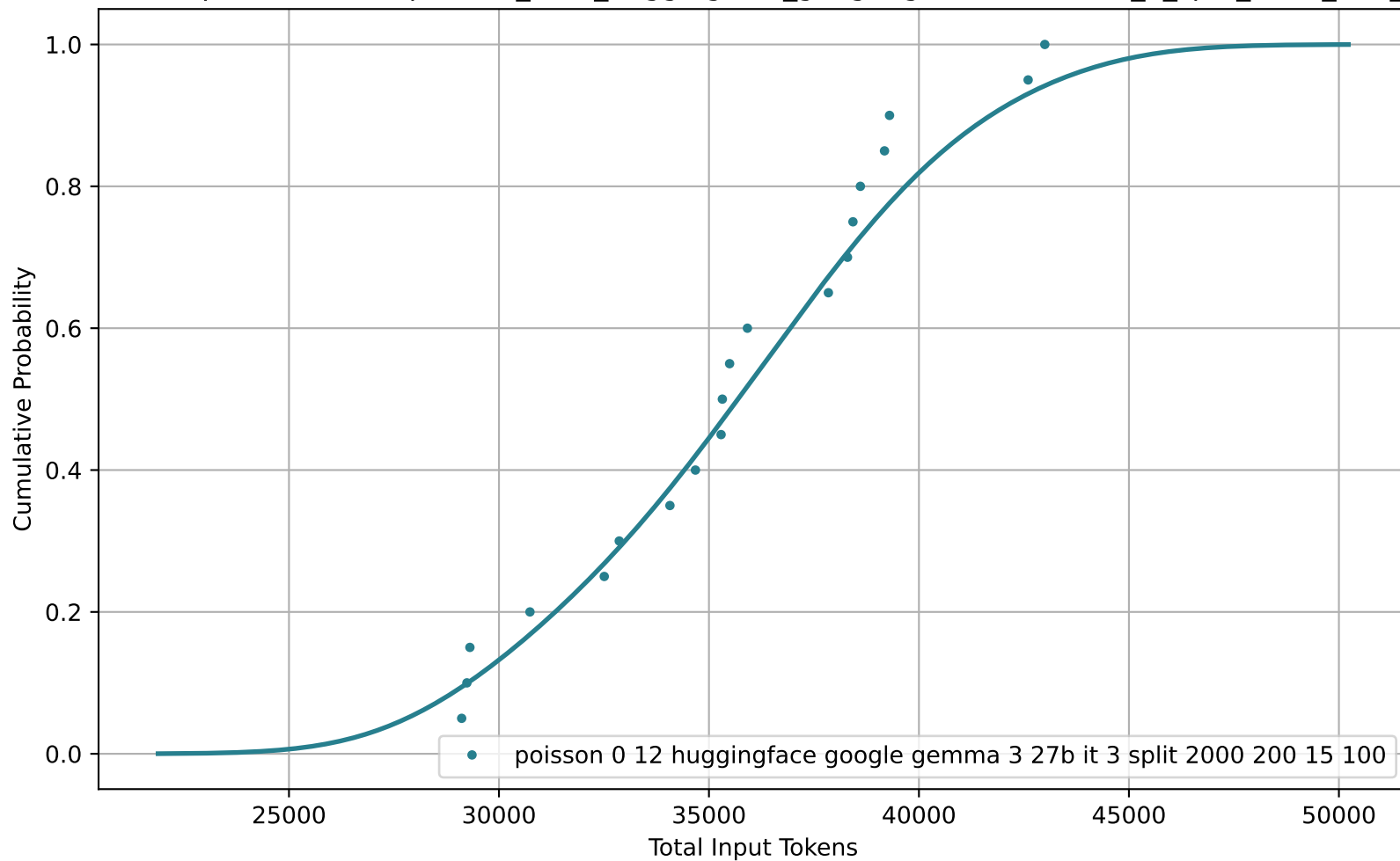
CDF of Total Input Tokens for poisson_0-12_huggingface_google-gemma-3-27b-it_3_split_2000_200_15_100
