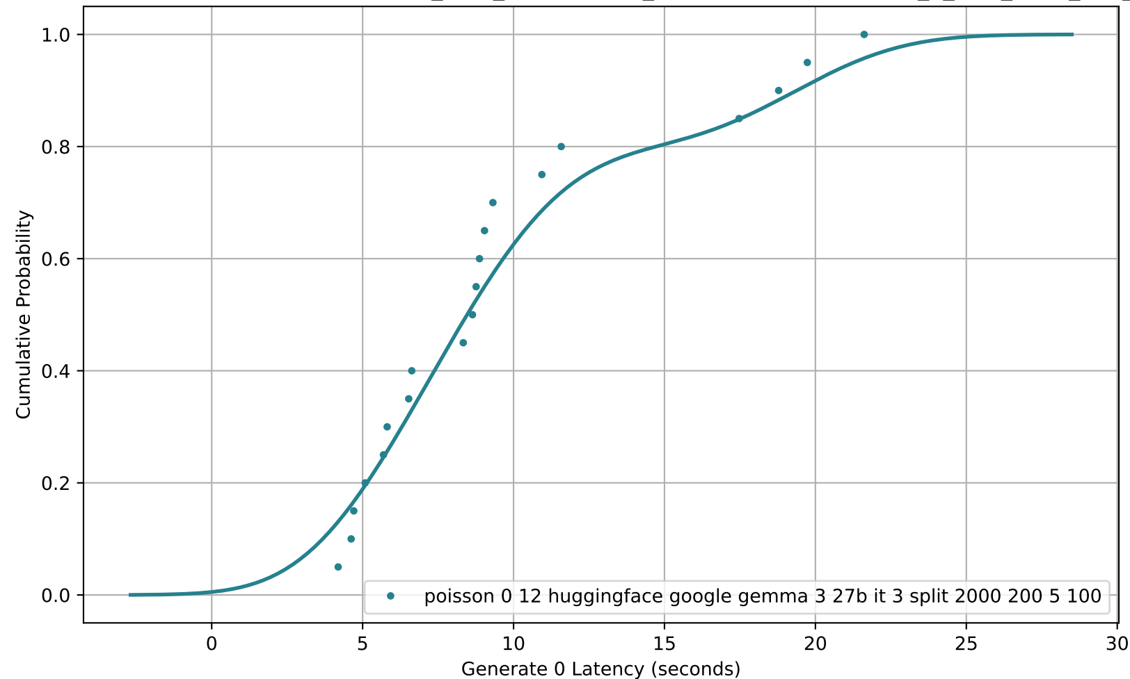
CDF of Generate 0 Latency for poisson_0-12_huggingface_google-gemma-3-27b-it_3_split_2000_200_5_100
