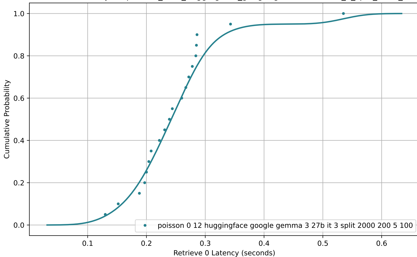
CDF of Retrieve 0 Latency for poisson_0-12_huggingface_google-gemma-3-27b-it_3_split_2000_200_5_100
