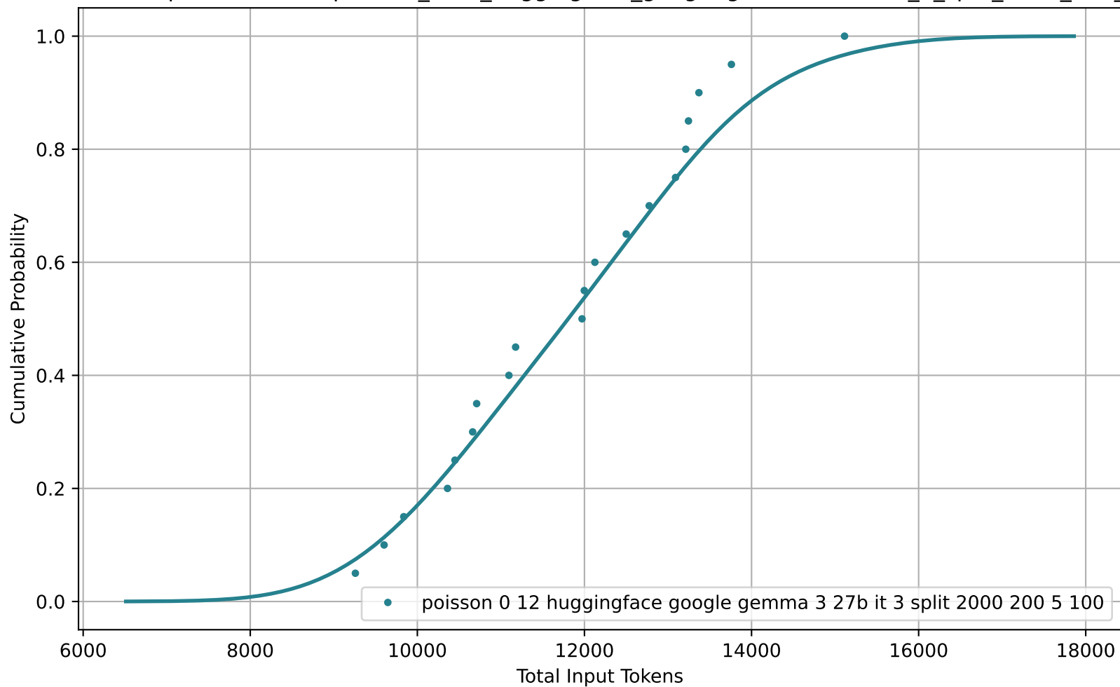
CDF of Total Input Tokens for poisson_0-12_huggingface_google-gemma-3-27b-it_3_split_2000_200_5_100
