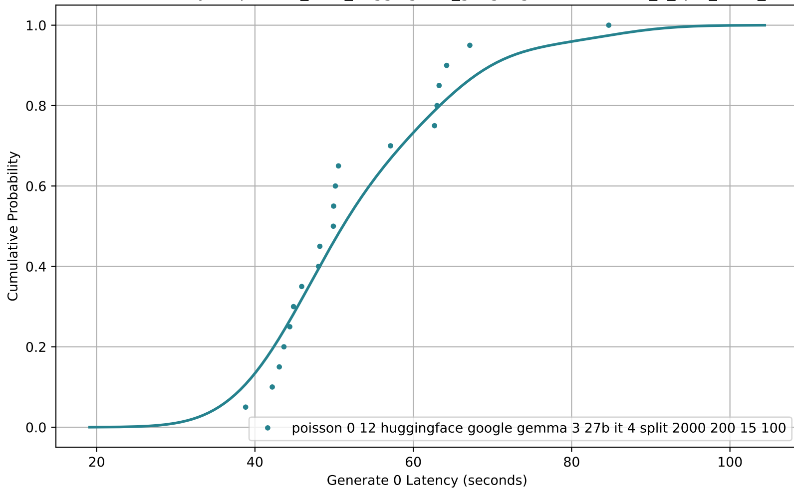
CDF of Generate 0 Latency for poisson_0-12_huggingface_google-gemma-3-27b-it_4_split_2000_200_15_100
