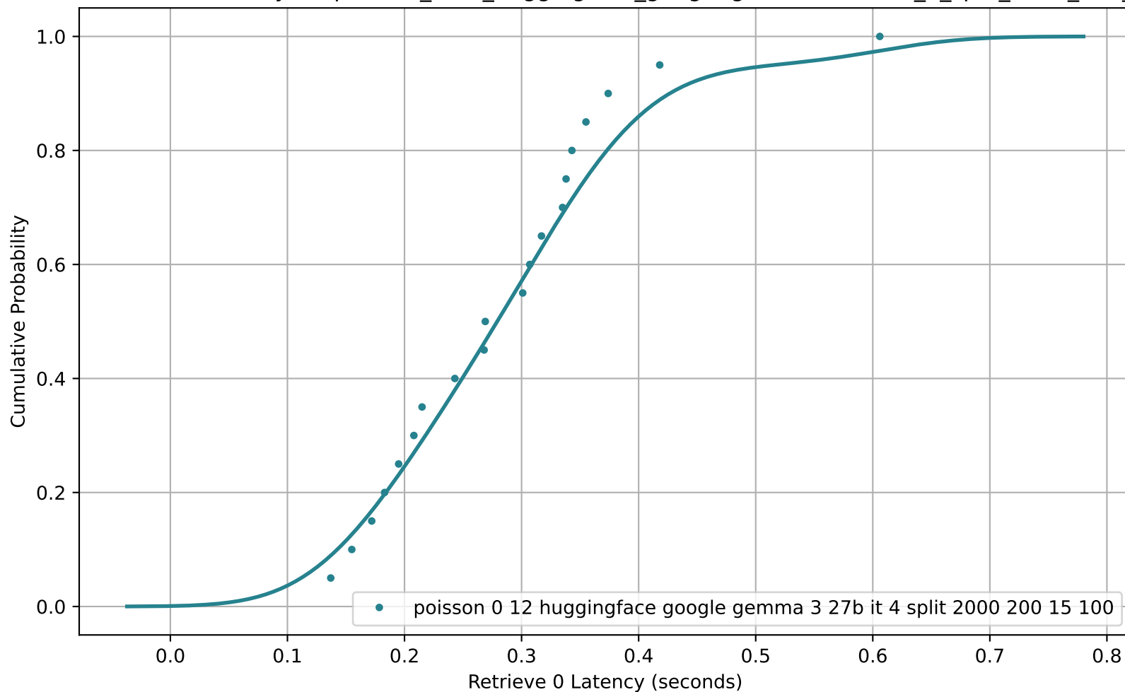
CDF of Retrieve 0 Latency for poisson_0-12_huggingface_google-gemma-3-27b-it_4_split_2000_200_15_100
