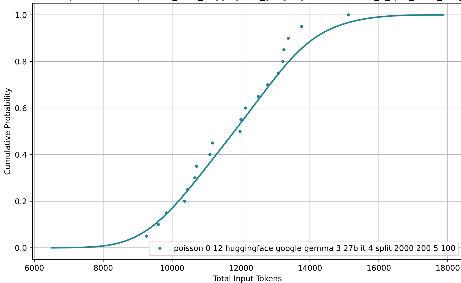
CDF of Total Input Tokens for poisson_0-12_huggingface_google-gemma-3-27b-it_4_split_2000_200_5_100
