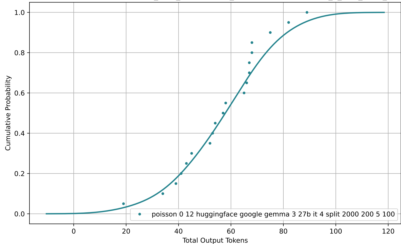
CDF of Total Output Tokens for poisson_0-12_huggingface_google-gemma-3-27b-it_4_split_2000_200_5_100
