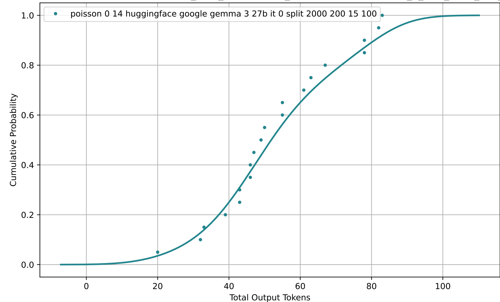
CDF of Total Output Tokens for poisson_0-14_huggingface_google-gemma-3-27b-it_0_split_2000_200_15_100
