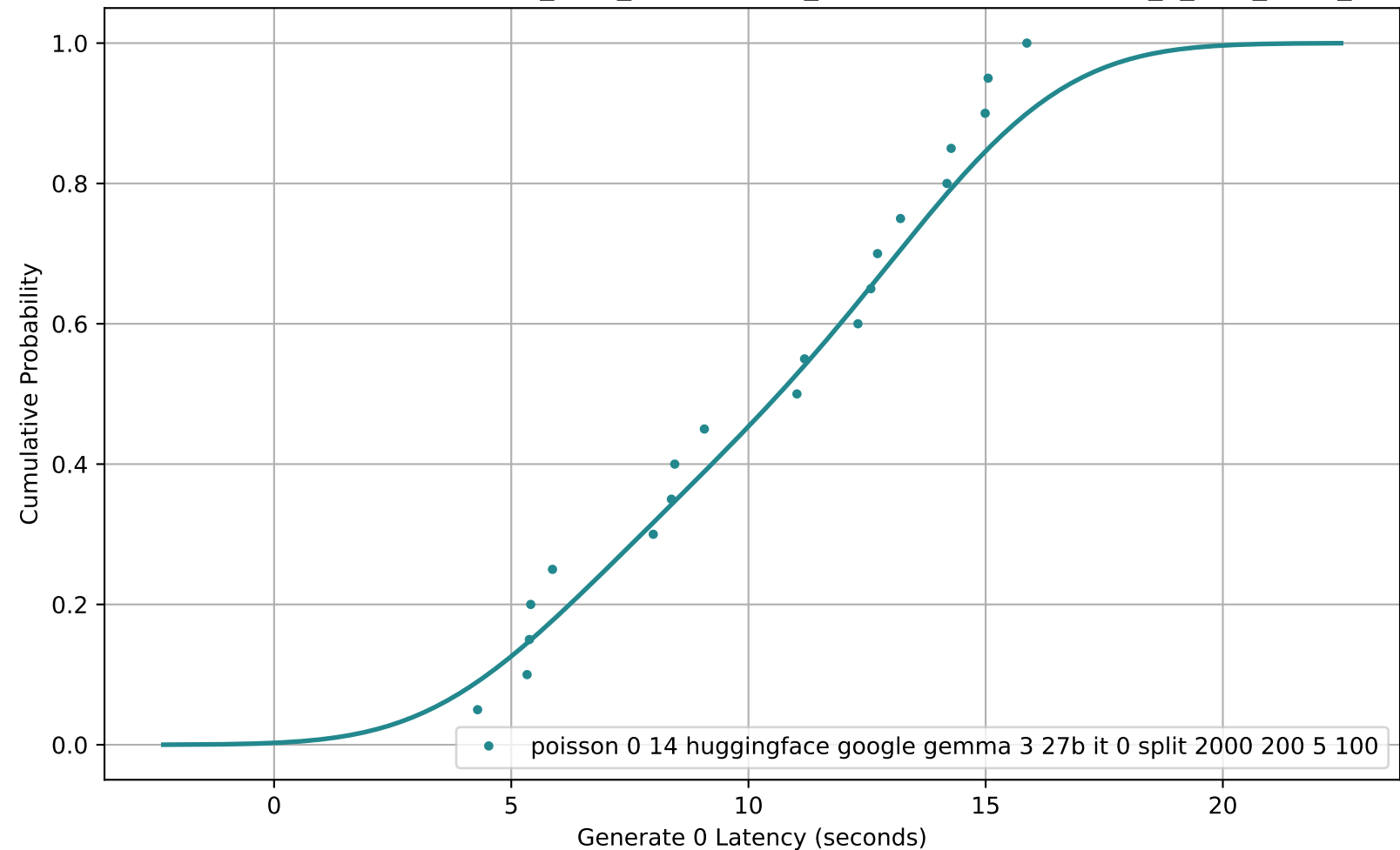
CDF of Generate 0 Latency for poisson_0-14_huggingface_google-gemma-3-27b-it_0_split_2000_200_5_100
