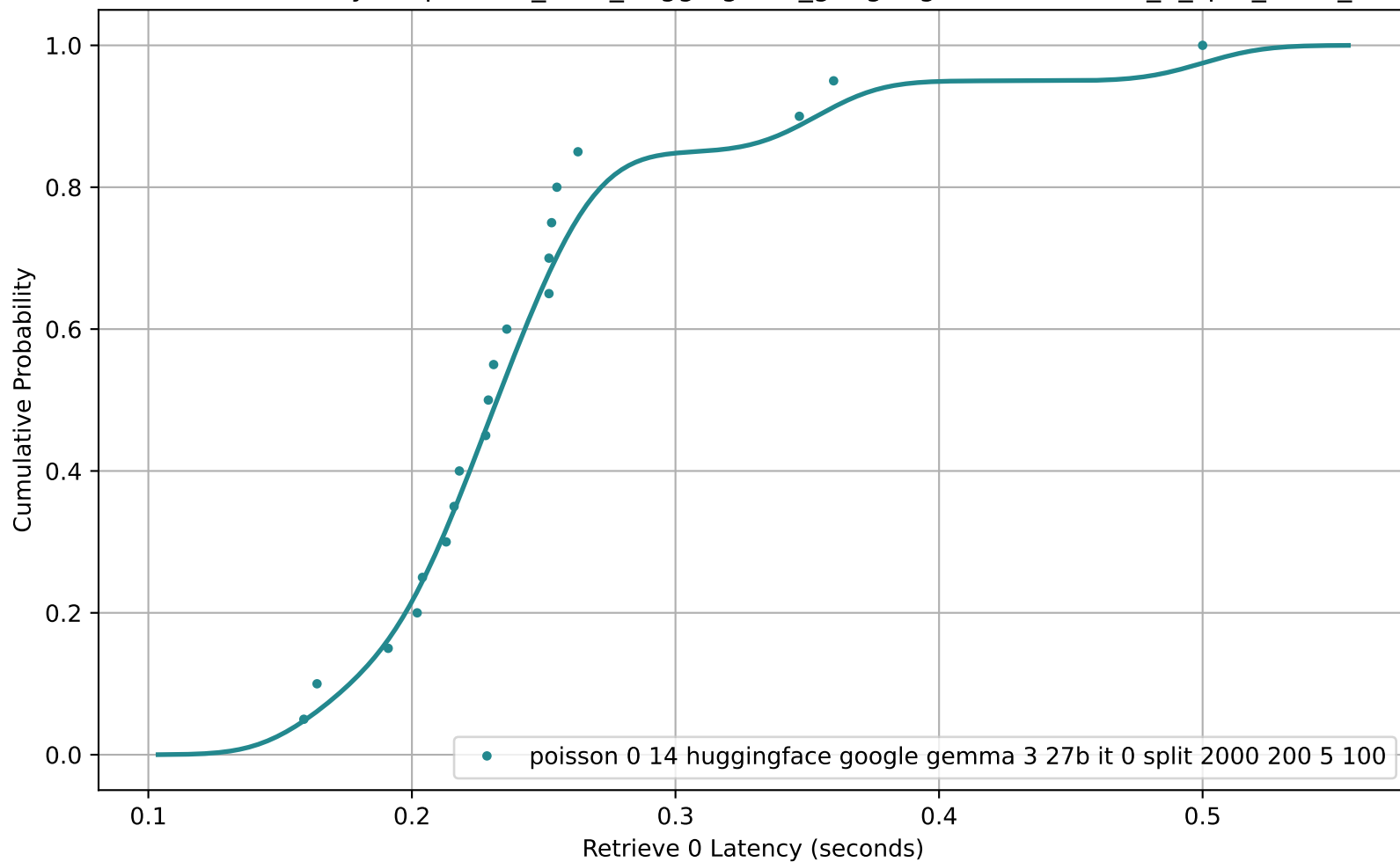
CDF of Retrieve 0 Latency for poisson_0-14_huggingface_google-gemma-3-27b-it_0_split_2000_200_5_100
