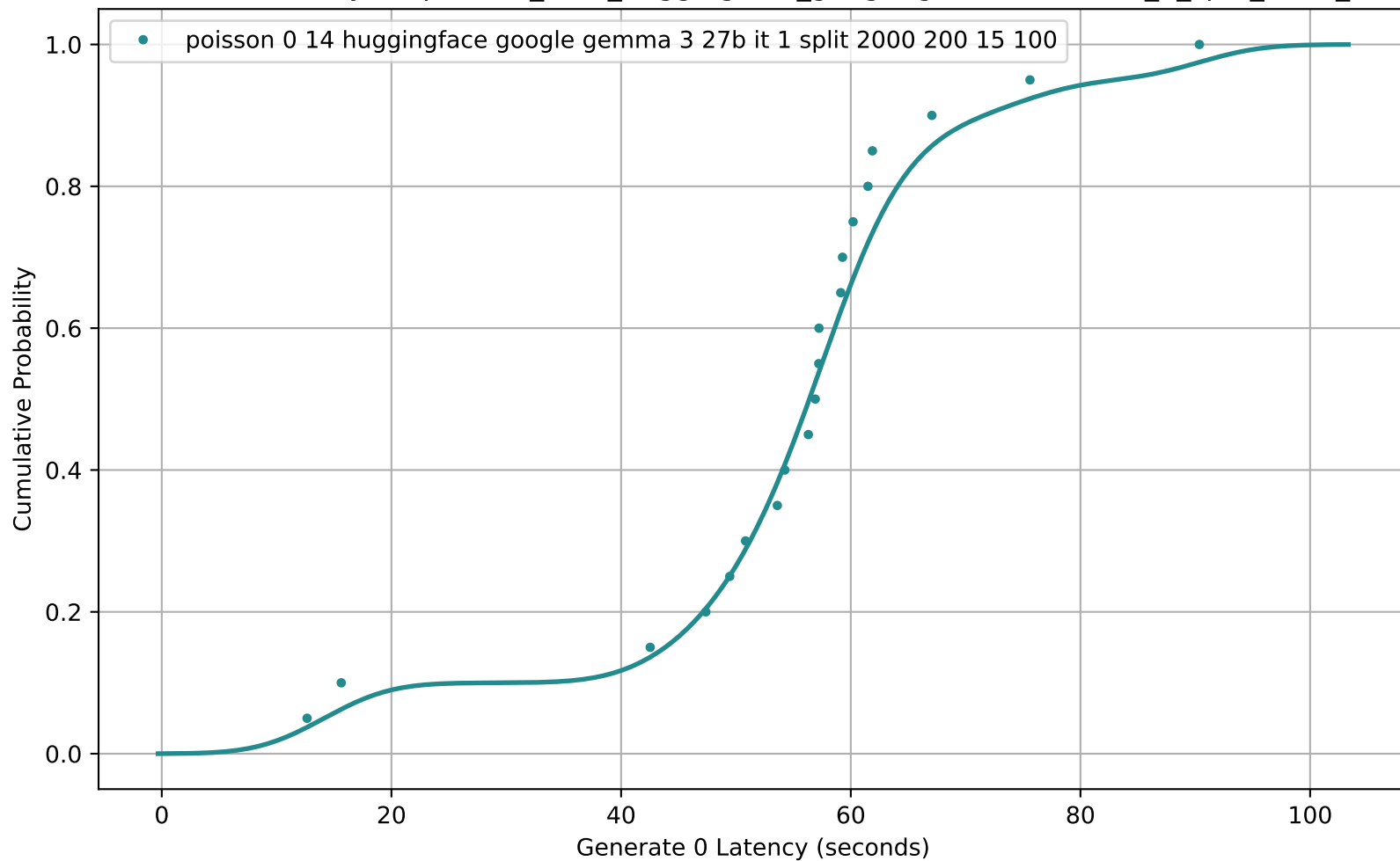
CDF of Generate 0 Latency for poisson_0-14_huggingface_google-gemma-3-27b-it_1_split_2000_200_15_100
