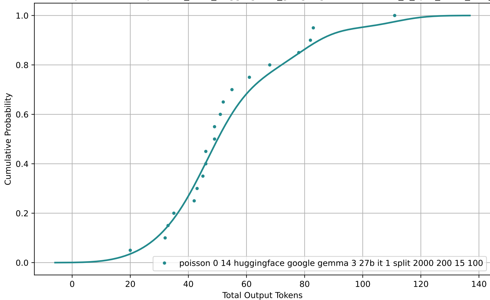
CDF of Total Output Tokens for poisson_0-14_huggingface_google-gemma-3-27b-it_1_split_2000_200_15_100
