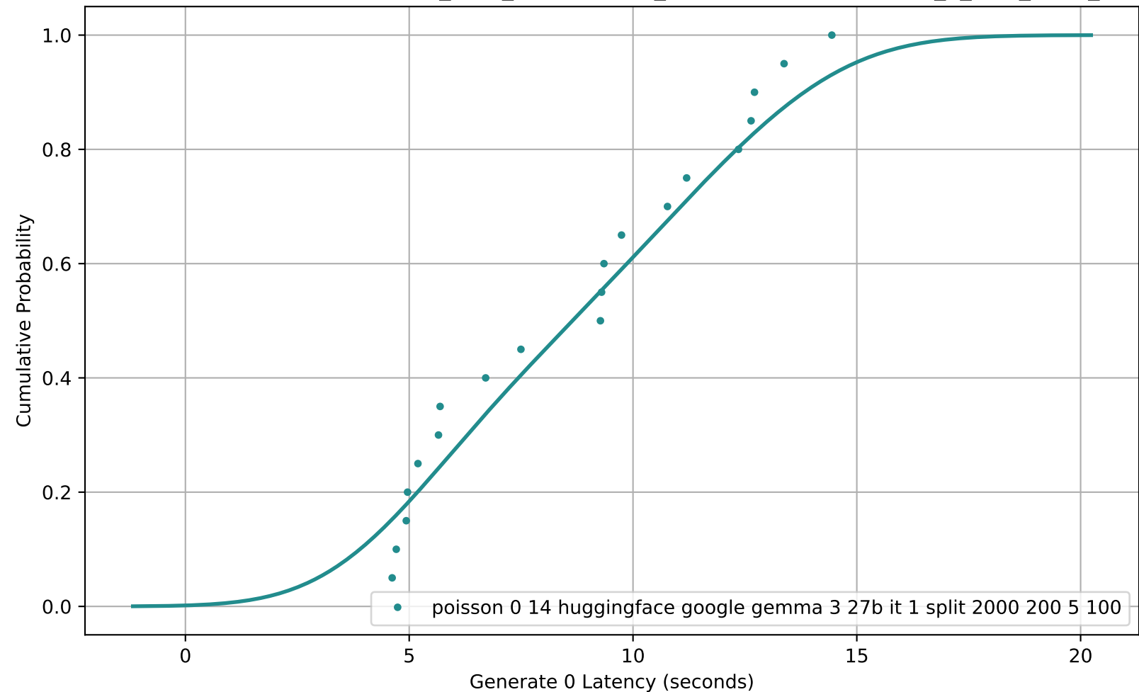
CDF of Generate 0 Latency for poisson_0-14_huggingface_google-gemma-3-27b-it_1_split_2000_200_5_100
