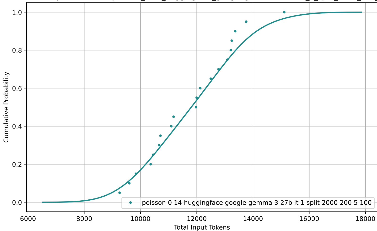
CDF of Total Input Tokens for poisson_0-14_huggingface_google-gemma-3-27b-it_1_split_2000_200_5_100
