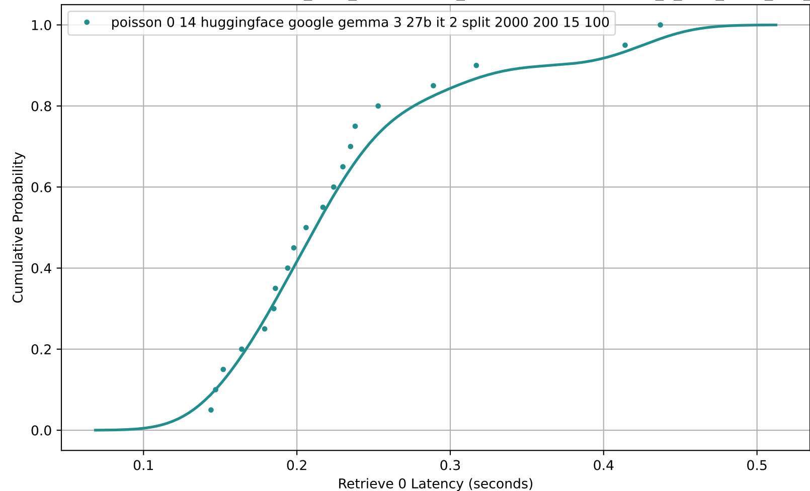
CDF of Retrieve 0 Latency for poisson_0-14_huggingface_google-gemma-3-27b-it_2_split_2000_200_15_100
