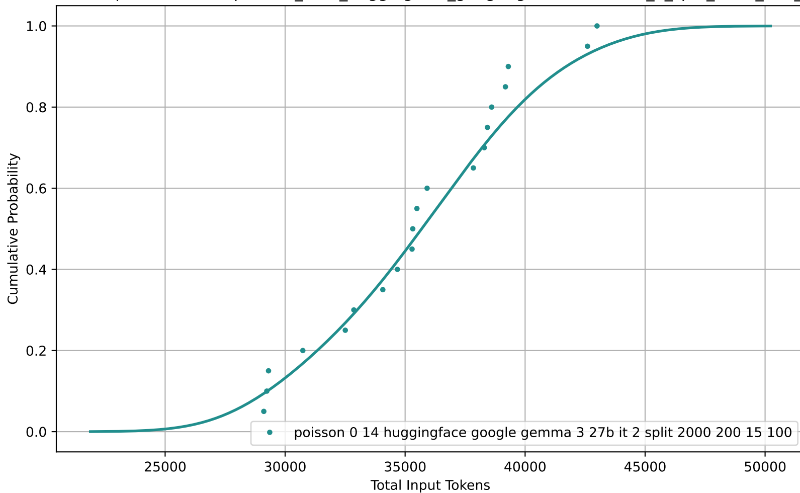
CDF of Total Input Tokens for poisson_0-14_huggingface_google-gemma-3-27b-it_2_split_2000_200_15_100
