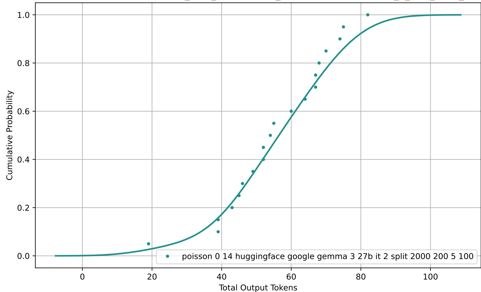
CDF of Total Output Tokens for poisson_0-14_huggingface_google-gemma-3-27b-it_2_split_2000_200_5_100
