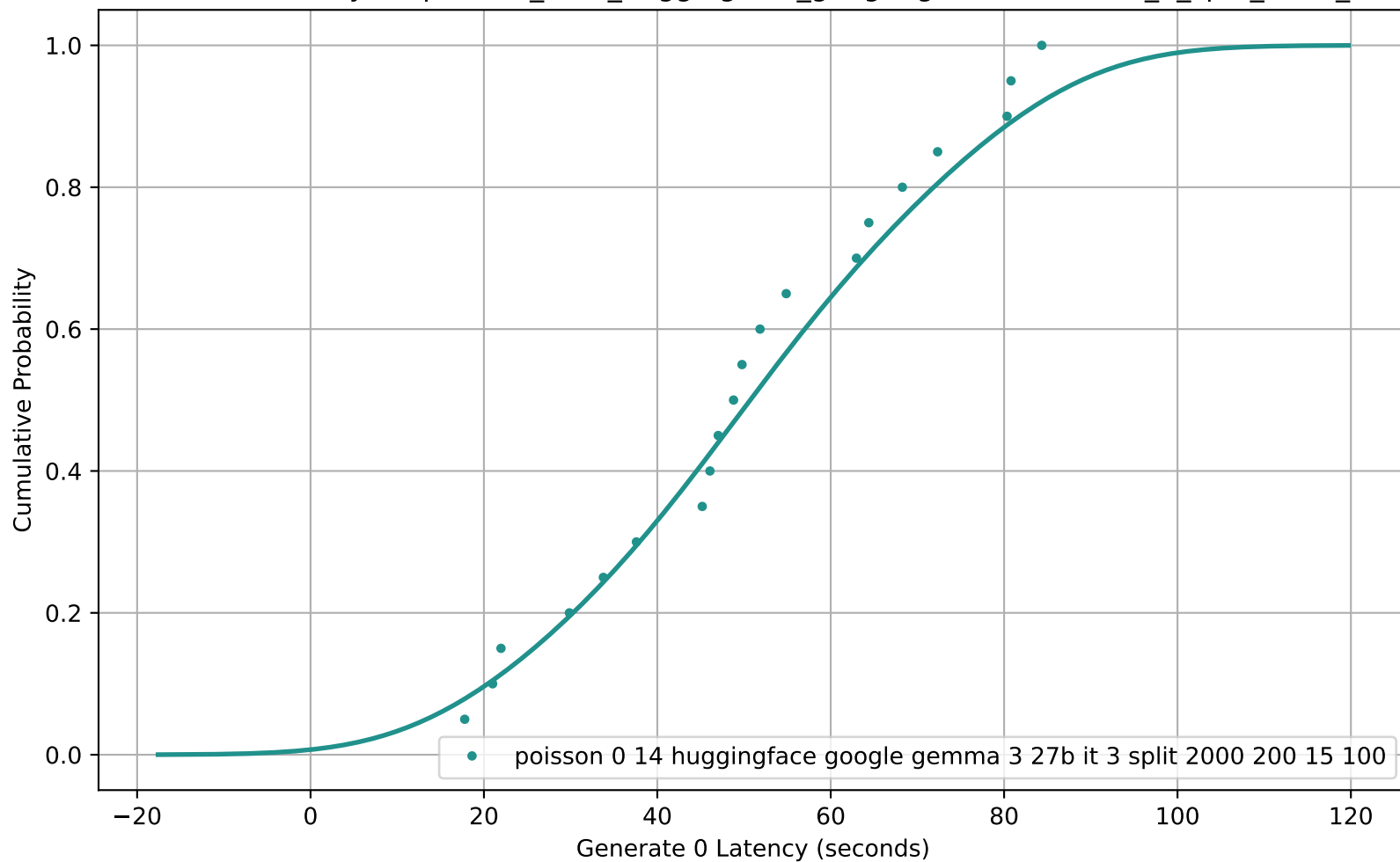
CDF of Generate 0 Latency for poisson_0-14_huggingface_google-gemma-3-27b-it_3_split_2000_200_15_100
