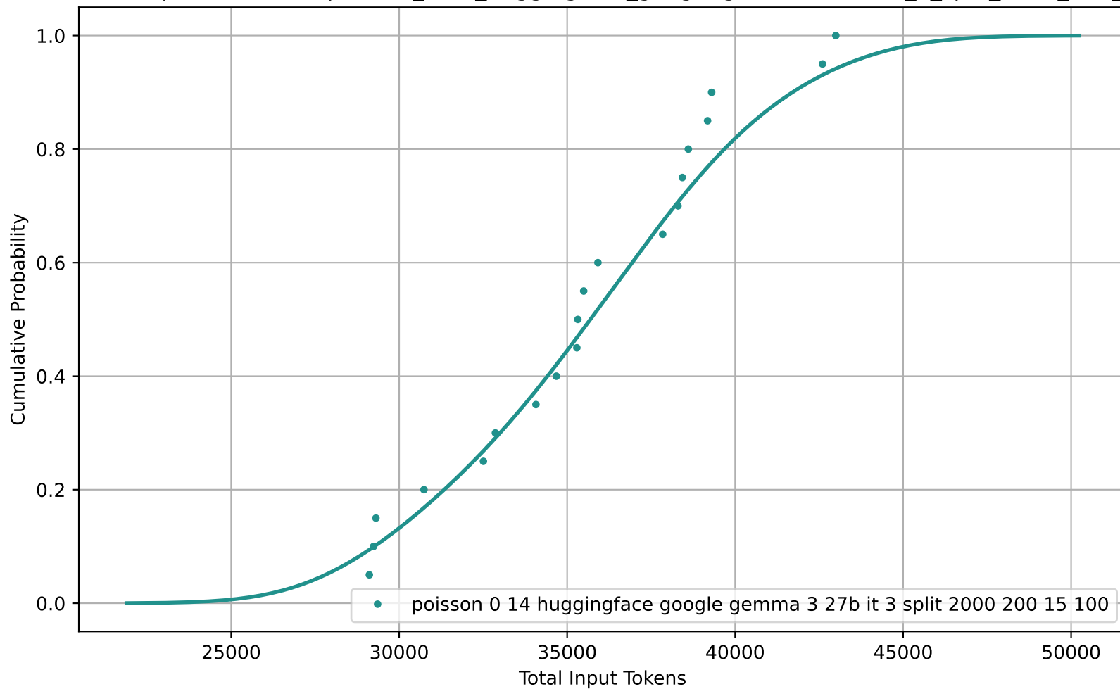
CDF of Total Input Tokens for poisson_0-14_huggingface_google-gemma-3-27b-it_3_split_2000_200_15_100
