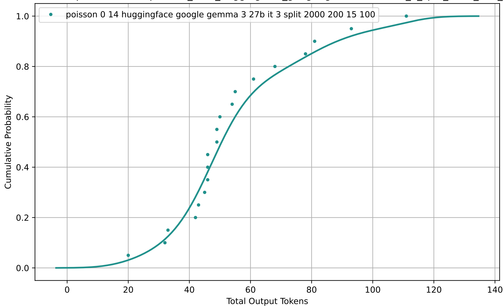
CDF of Total Output Tokens for poisson_0-14_huggingface_google-gemma-3-27b-it_3_split_2000_200_15_100
