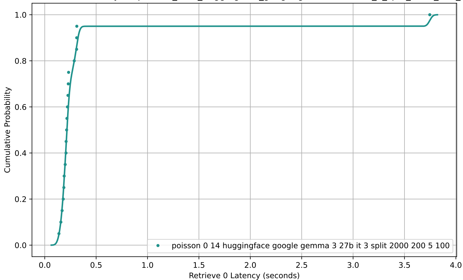
CDF of Retrieve 0 Latency for poisson_0-14_huggingface_google-gemma-3-27b-it_3_split_2000_200_5_100
