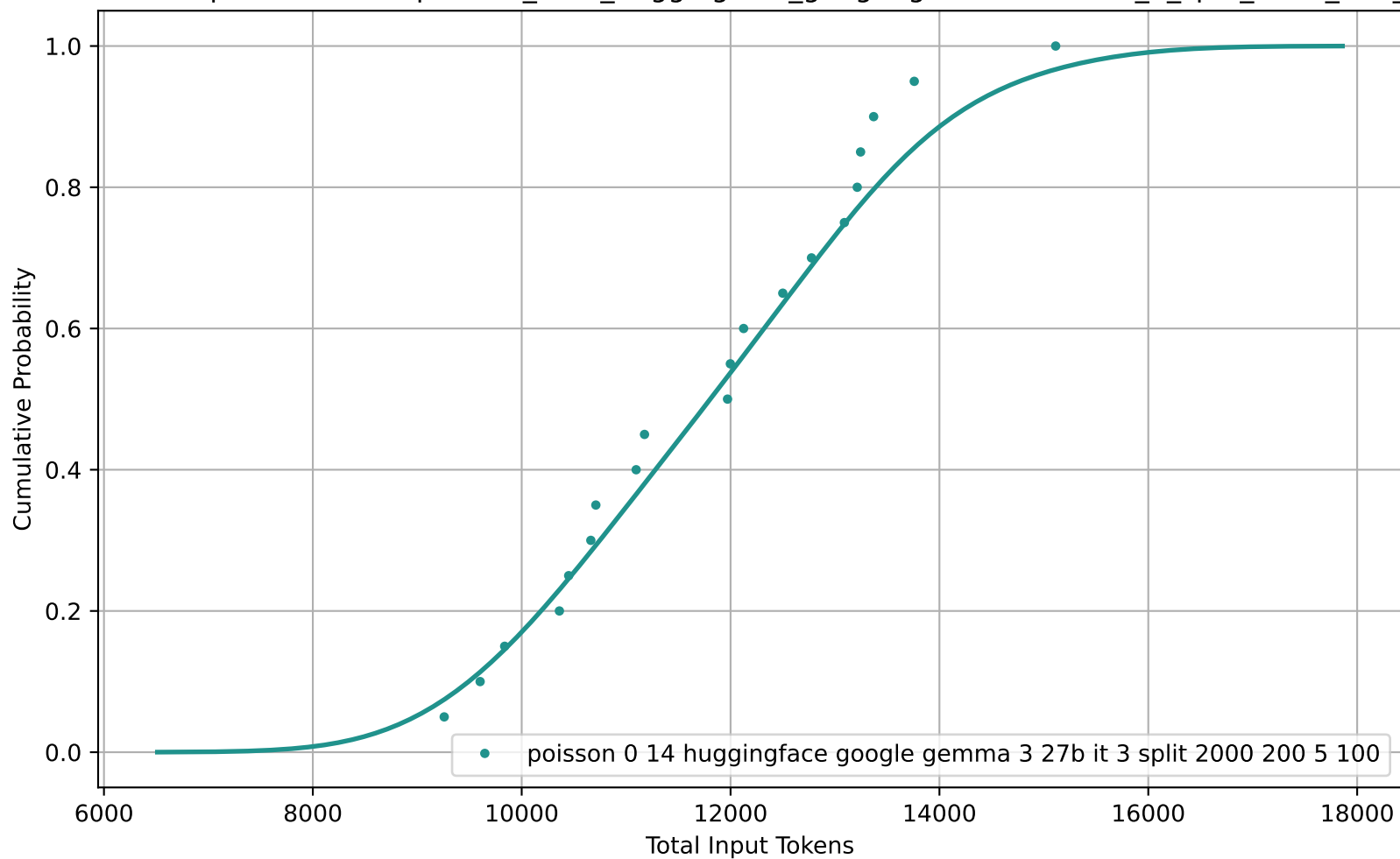
CDF of Total Input Tokens for poisson_0-14_huggingface_google-gemma-3-27b-it_3_split_2000_200_5_100
