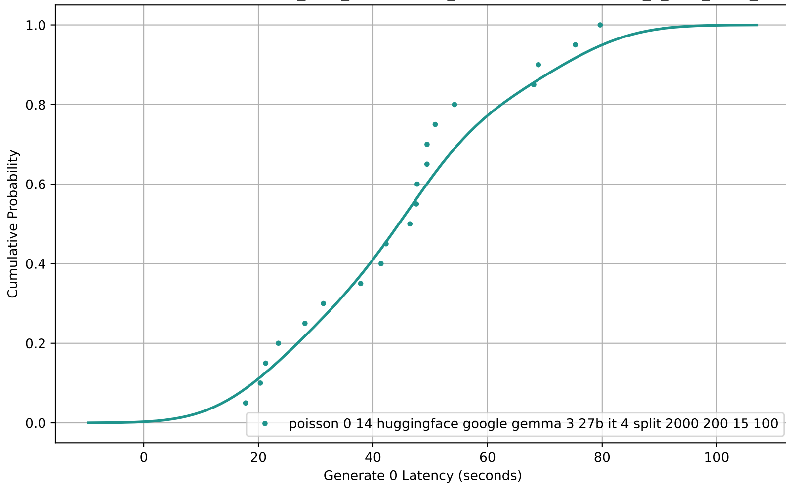
CDF of Generate 0 Latency for poisson_0-14_huggingface_google-gemma-3-27b-it_4_split_2000_200_15_100
