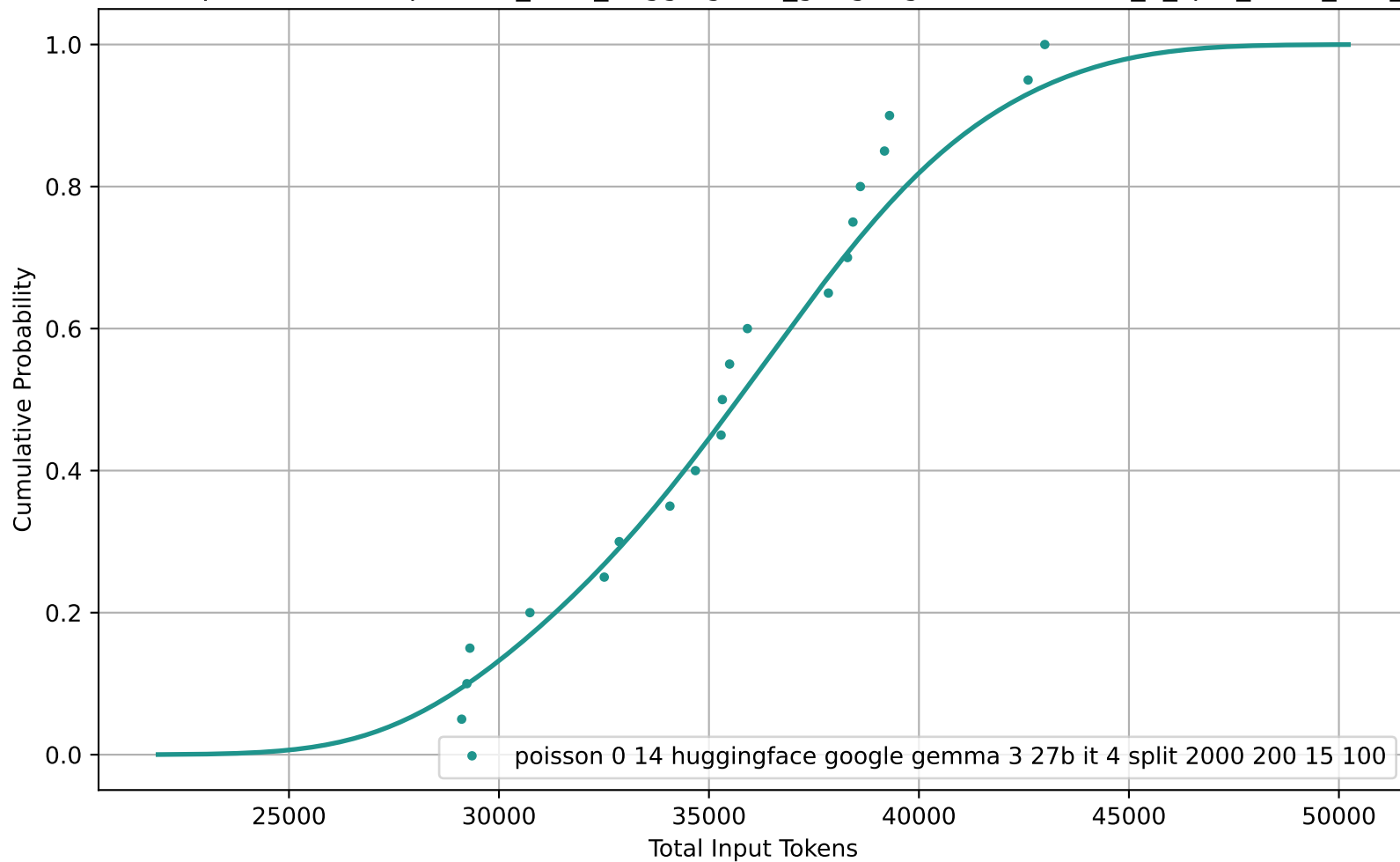
CDF of Total Input Tokens for poisson_0-14_huggingface_google-gemma-3-27b-it_4_split_2000_200_15_100
