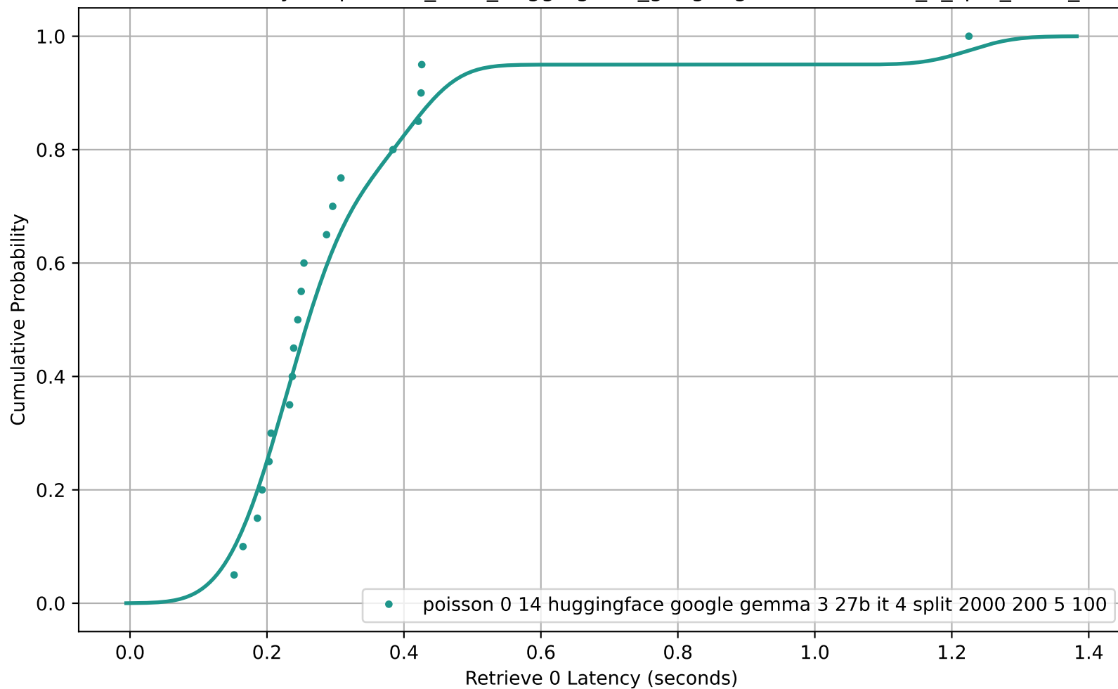
CDF of Retrieve 0 Latency for poisson_0-14_huggingface_google-gemma-3-27b-it_4_split_2000_200_5_100
