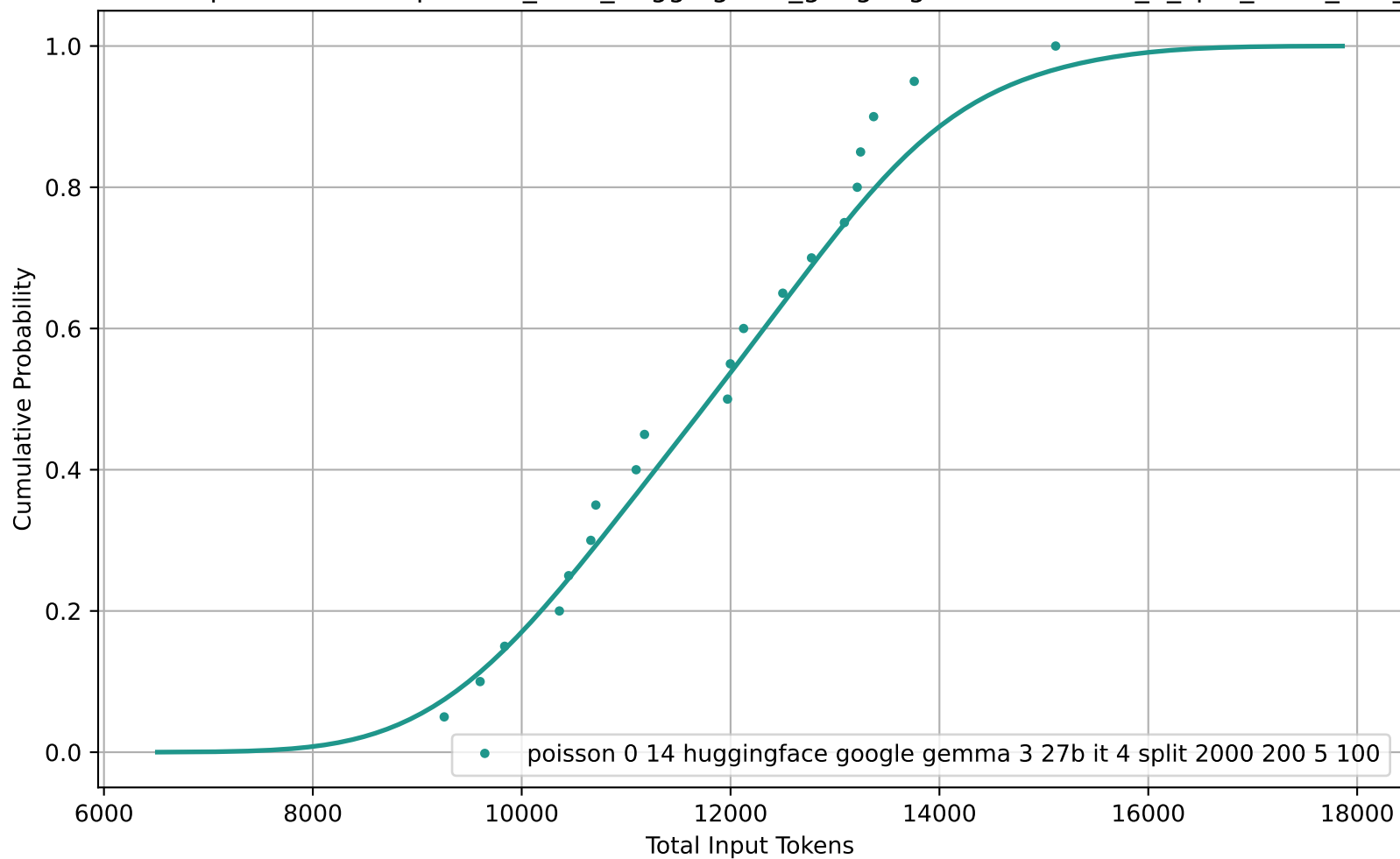
CDF of Total Input Tokens for poisson_0-14_huggingface_google-gemma-3-27b-it_4_split_2000_200_5_100
