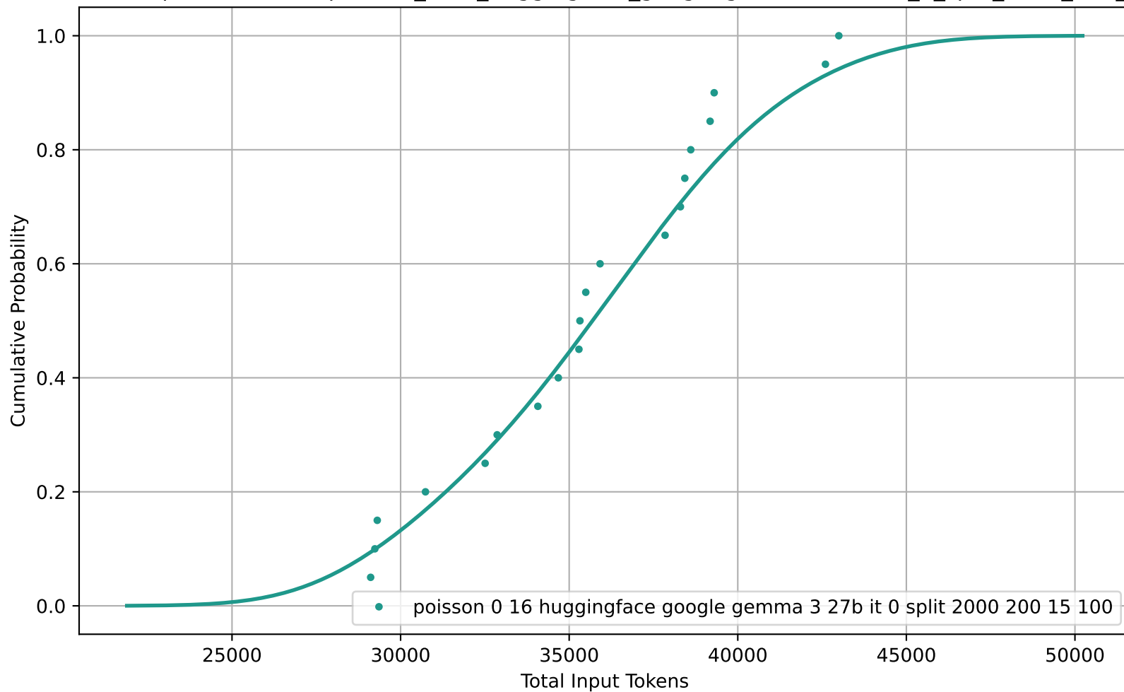
CDF of Total Input Tokens for poisson_0-16_huggingface_google-gemma-3-27b-it_0_split_2000_200_15_100
