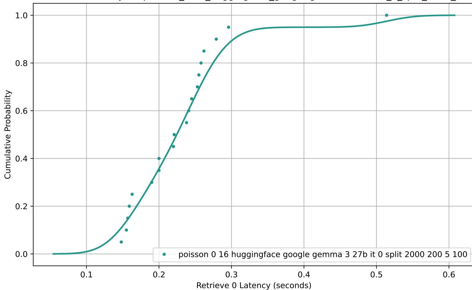
CDF of Retrieve 0 Latency for poisson_0-16_huggingface_google-gemma-3-27b-it_0_split_2000_200_5_100
