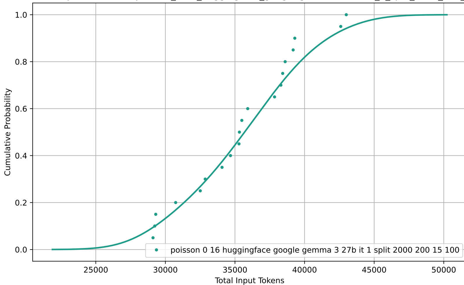
CDF of Total Input Tokens for poisson_0-16_huggingface_google-gemma-3-27b-it_1_split_2000_200_15_100
