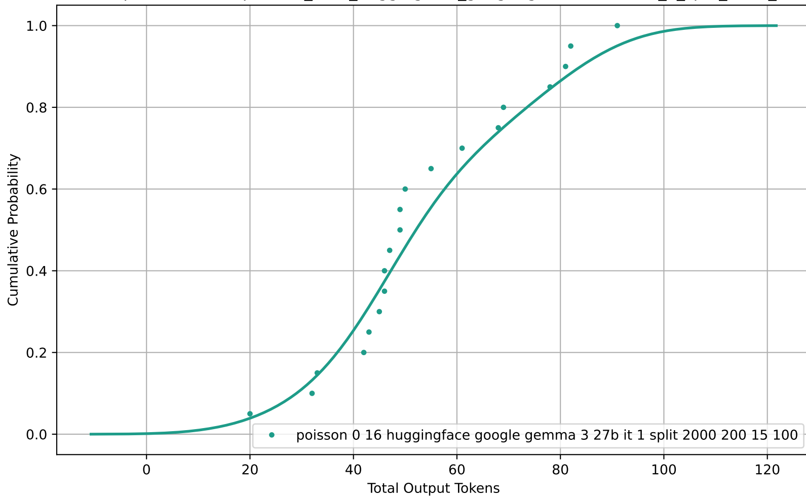
CDF of Total Output Tokens for poisson_0-16_huggingface_google-gemma-3-27b-it_1_split_2000_200_15_100
