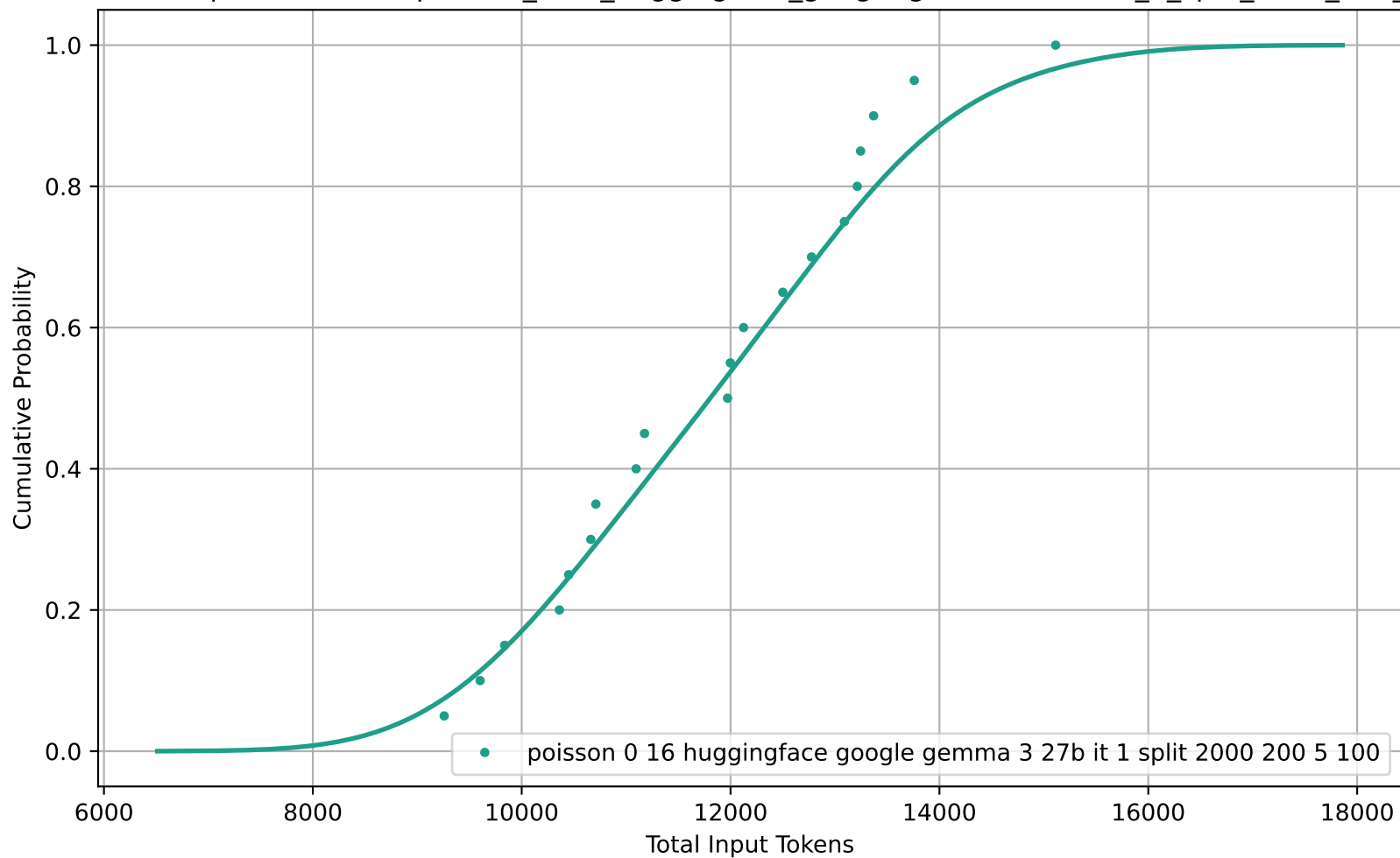
CDF of Total Input Tokens for poisson_0-16_huggingface_google-gemma-3-27b-it_1_split_2000_200_5_100
