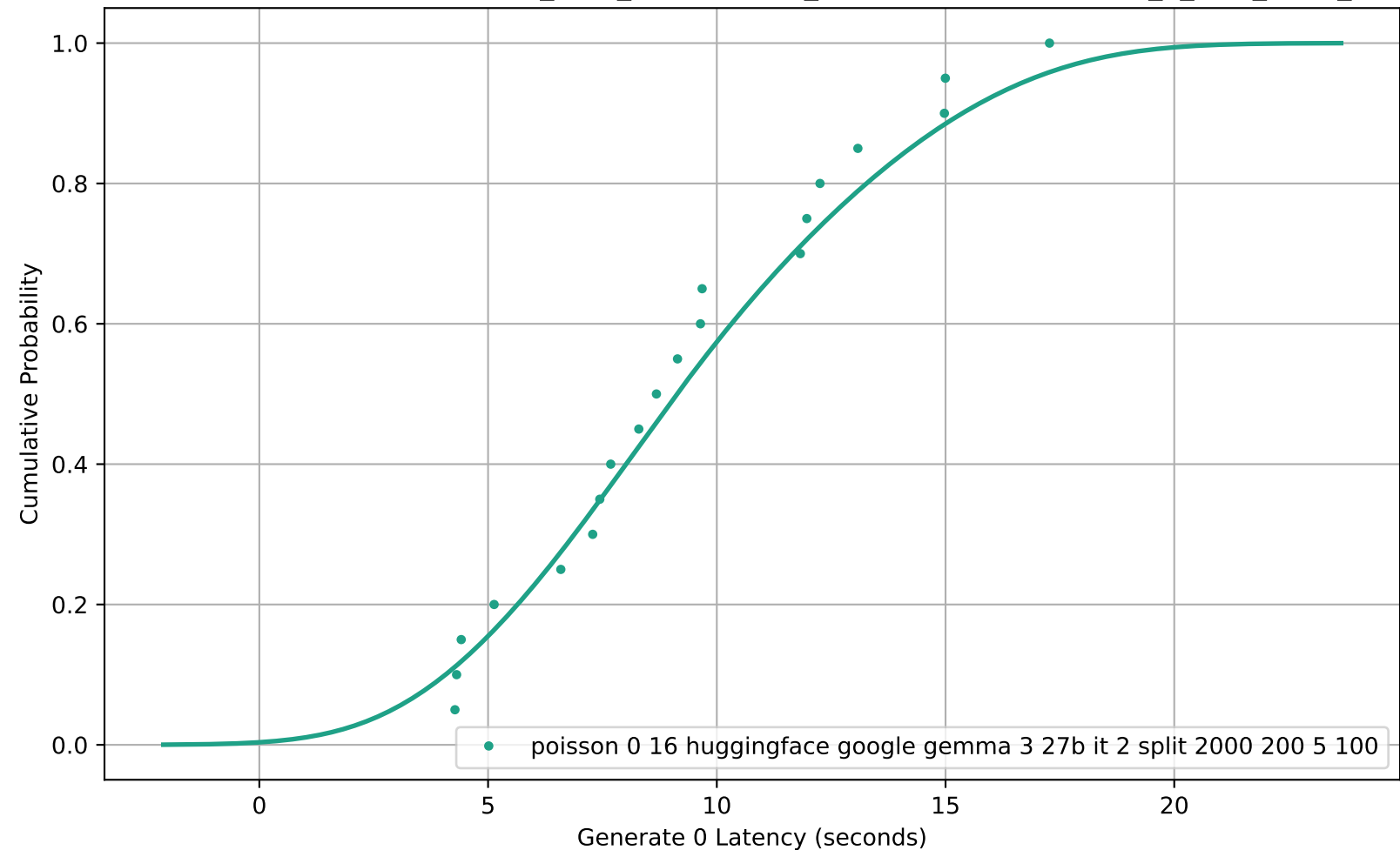
CDF of Generate 0 Latency for poisson_0-16_huggingface_google-gemma-3-27b-it_2_split_2000_200_5_100
