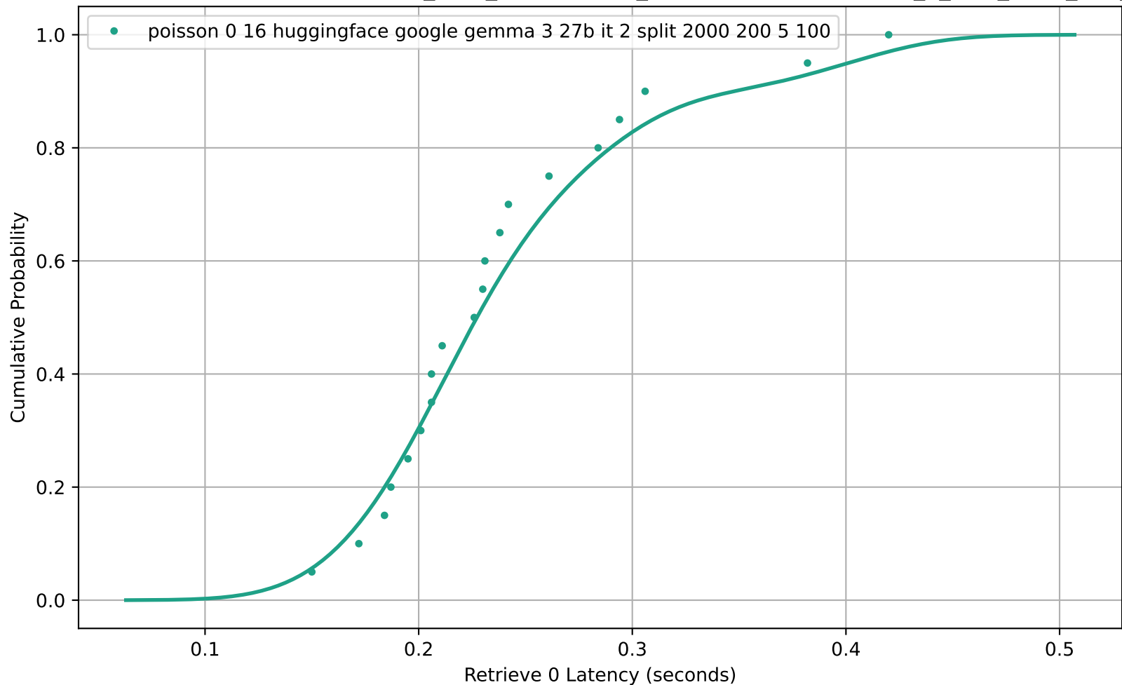
CDF of Retrieve 0 Latency for poisson_0-16_huggingface_google-gemma-3-27b-it_2_split_2000_200_5_100
