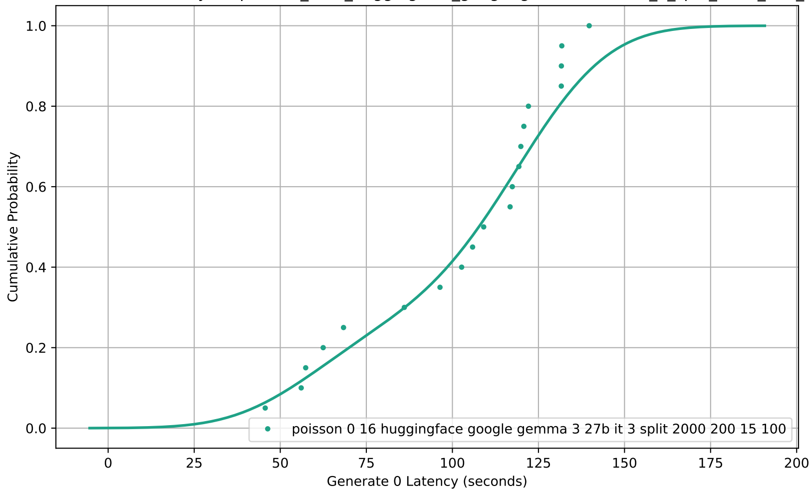
CDF of Generate 0 Latency for poisson_0-16_huggingface_google-gemma-3-27b-it_3_split_2000_200_15_100
