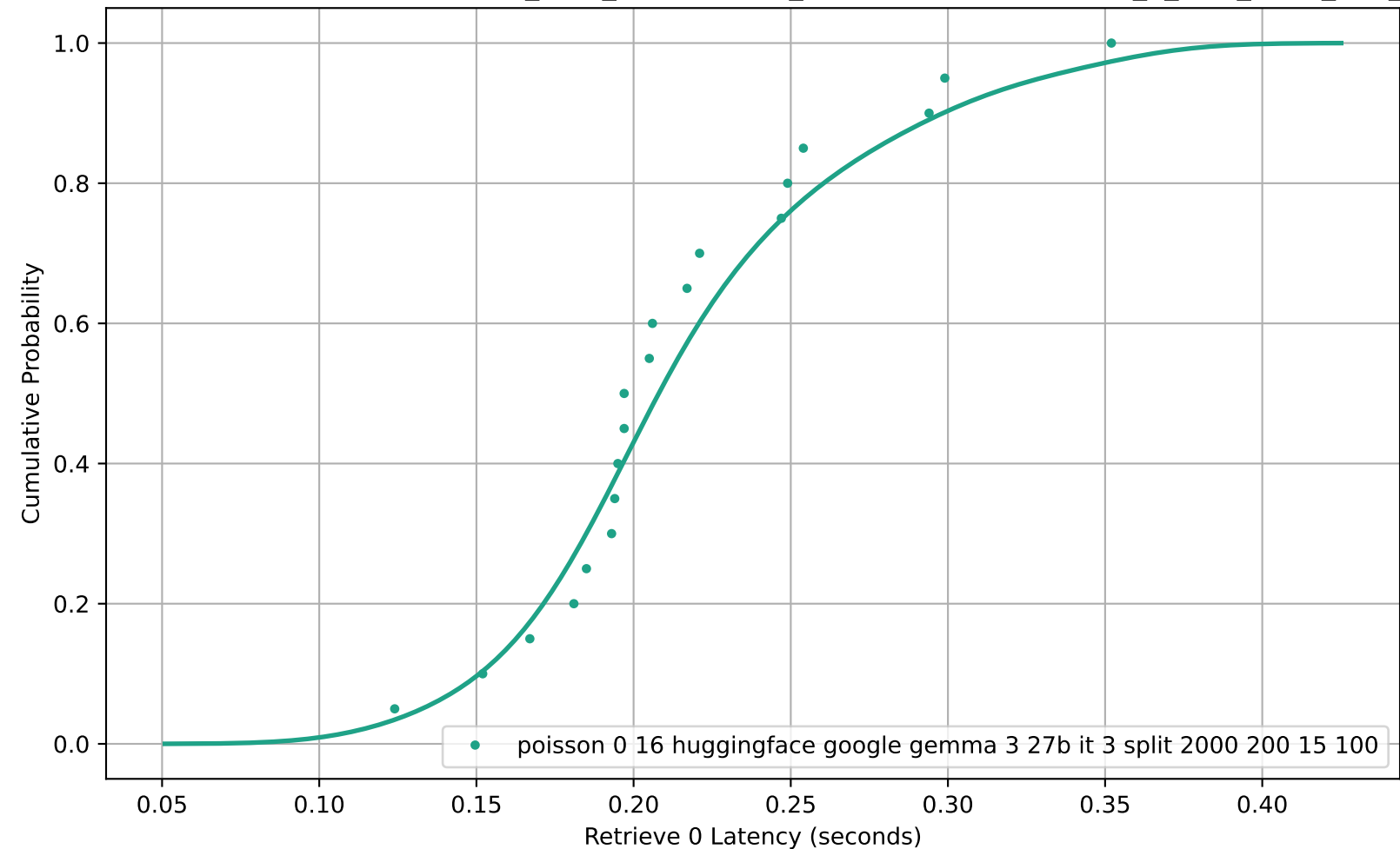
CDF of Retrieve 0 Latency for poisson_0-16_huggingface_google-gemma-3-27b-it_3_split_2000_200_15_100
