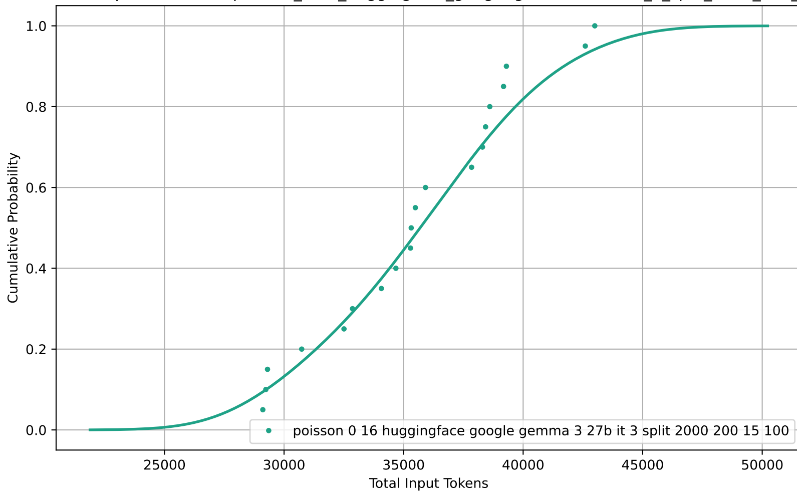
CDF of Total Input Tokens for poisson_0-16_huggingface_google-gemma-3-27b-it_3_split_2000_200_15_100
