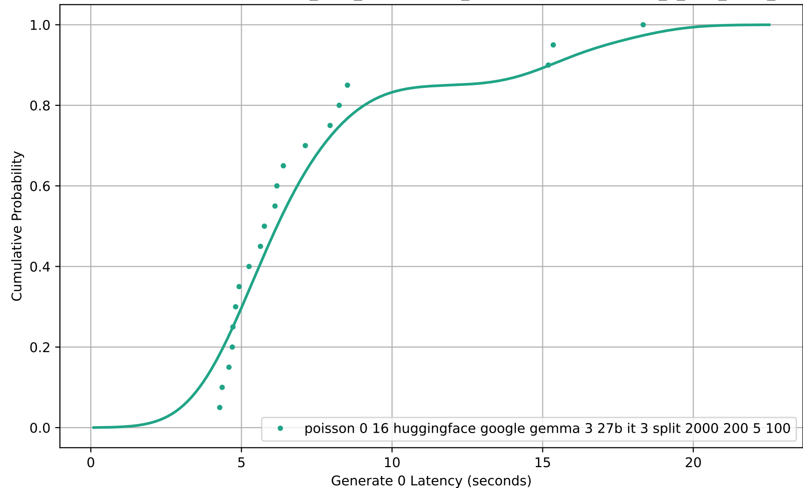
CDF of Generate 0 Latency for poisson_0-16_huggingface_google-gemma-3-27b-it_3_split_2000_200_5_100
